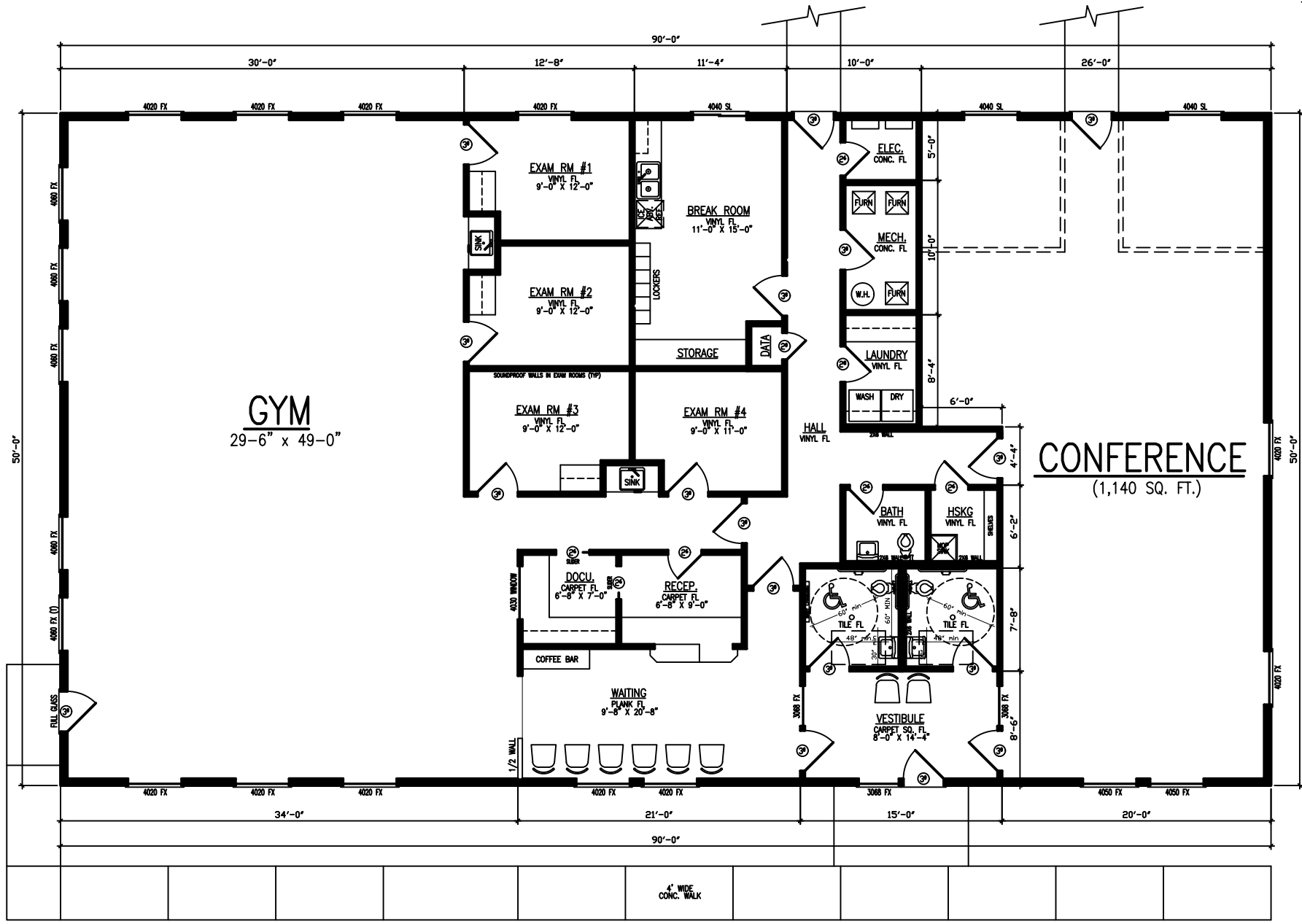
FLOOR PLAN SCALE: 1/4" = 1'-0" 3,360 SQ. FT. PT CLINIC 1,140 SQ. FT. CONFERENCE 4,500 SQ. FT. TOTAL
